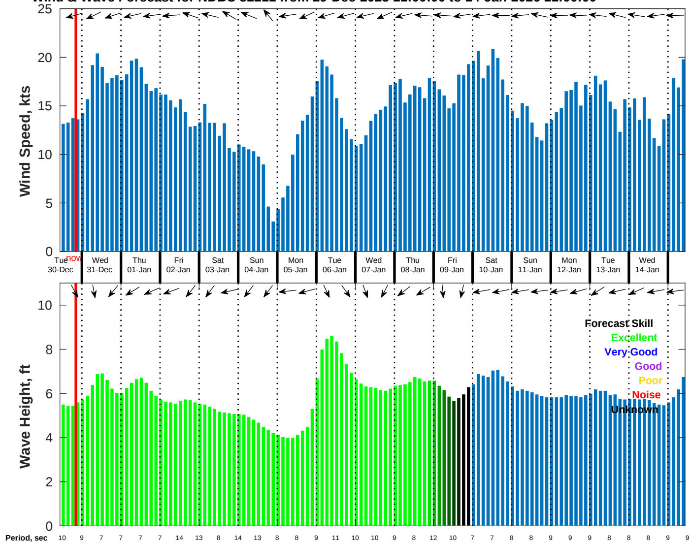
Wind & Wave Forecast for NDBC 52211 from 29-Dec-2025 11:00:00 to 14-Jan-2026 11:00:00
