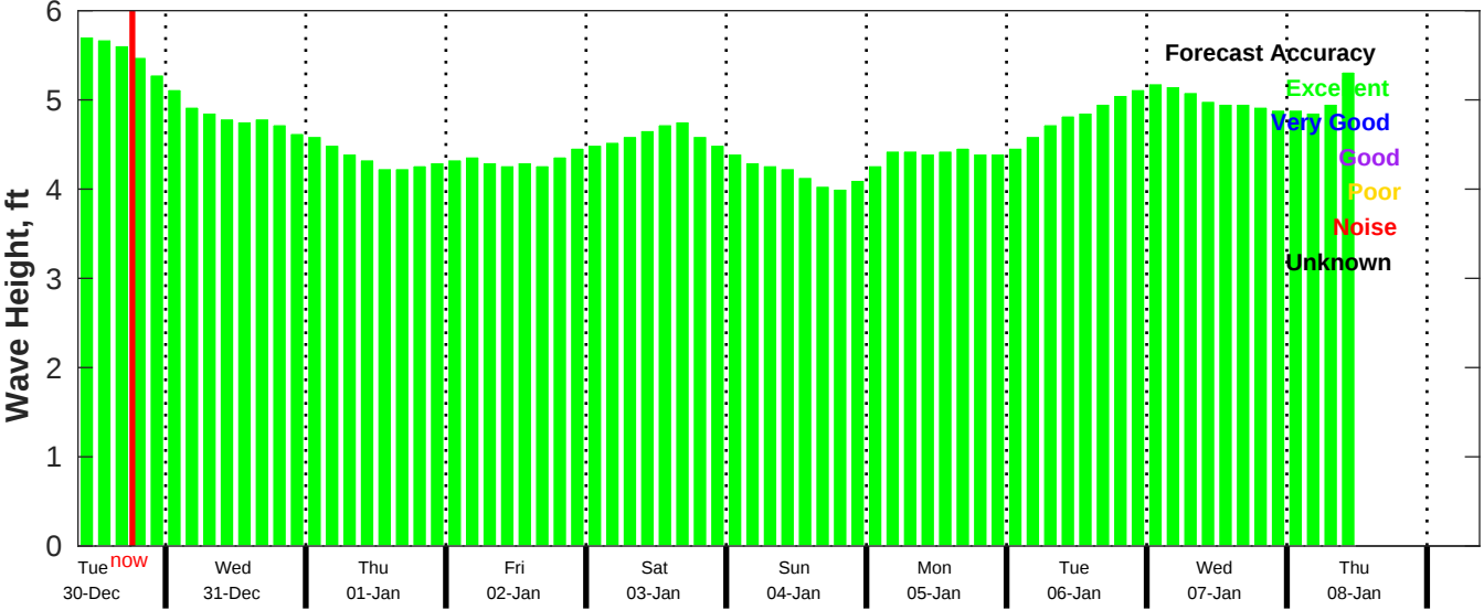
CMEMS Wave Forecast for NDBC 52212 from 29-Dec-2025 09:00:00 to 08-Jan-2026 09:00:00
