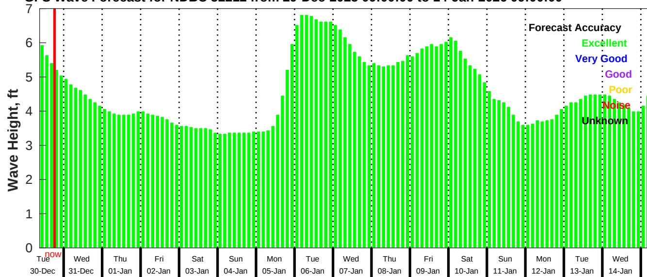
GFS Wave Forecast for NDBC 52212 from 29-Dec-2025 09:00:00 to 14-Jan-2026 09:00:00
