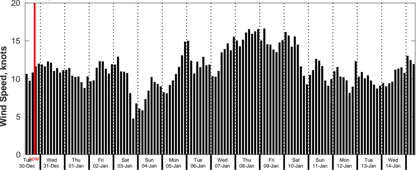
GFS Wind Speed Forecast for NDBC 52212 from 29-Dec-2025 09:00:00 to 14-Jan-2026 09:00:00
