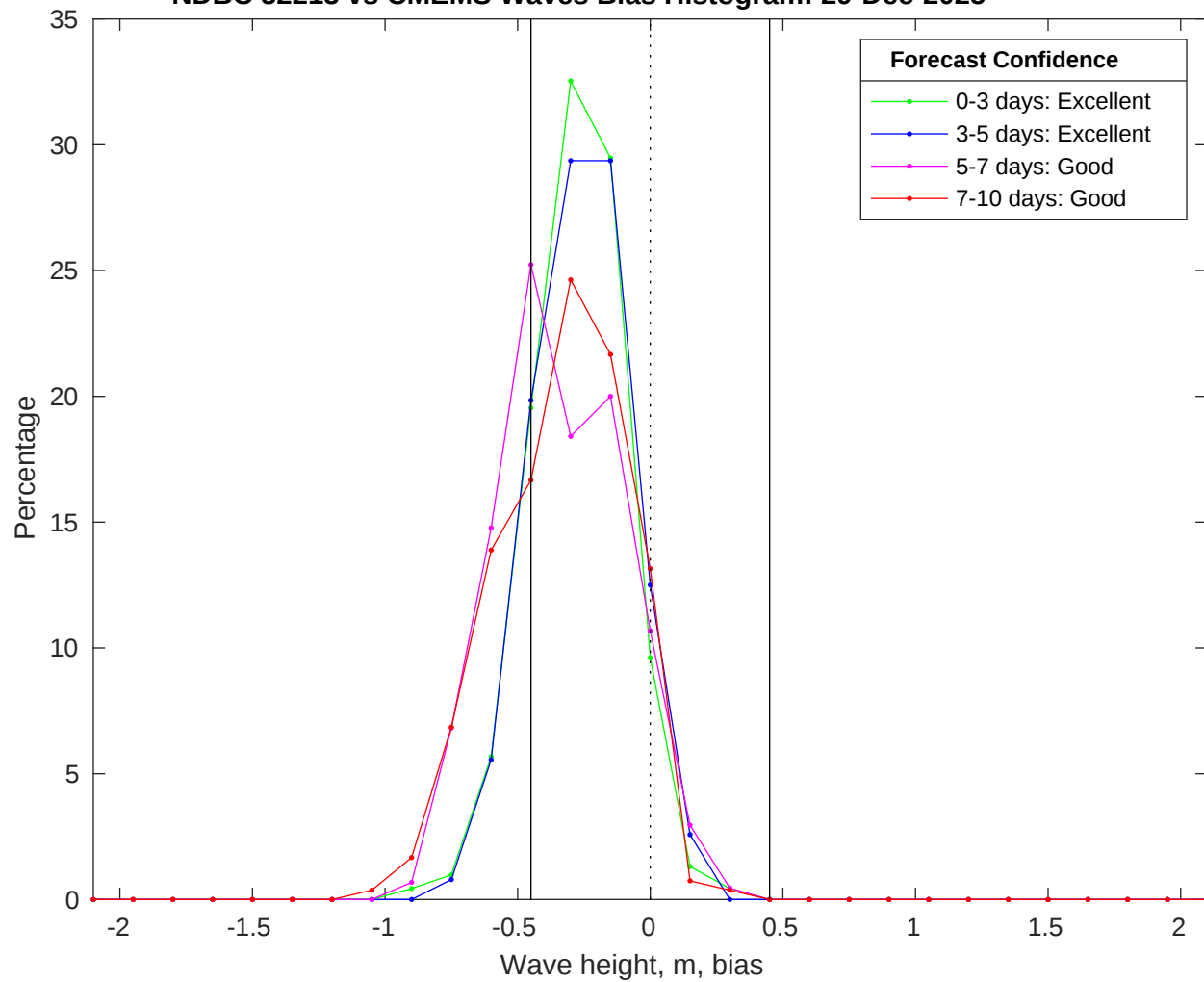
NDBC 52213 vs CMEMS Waves Bias Histogram: 29-Dec-2025
