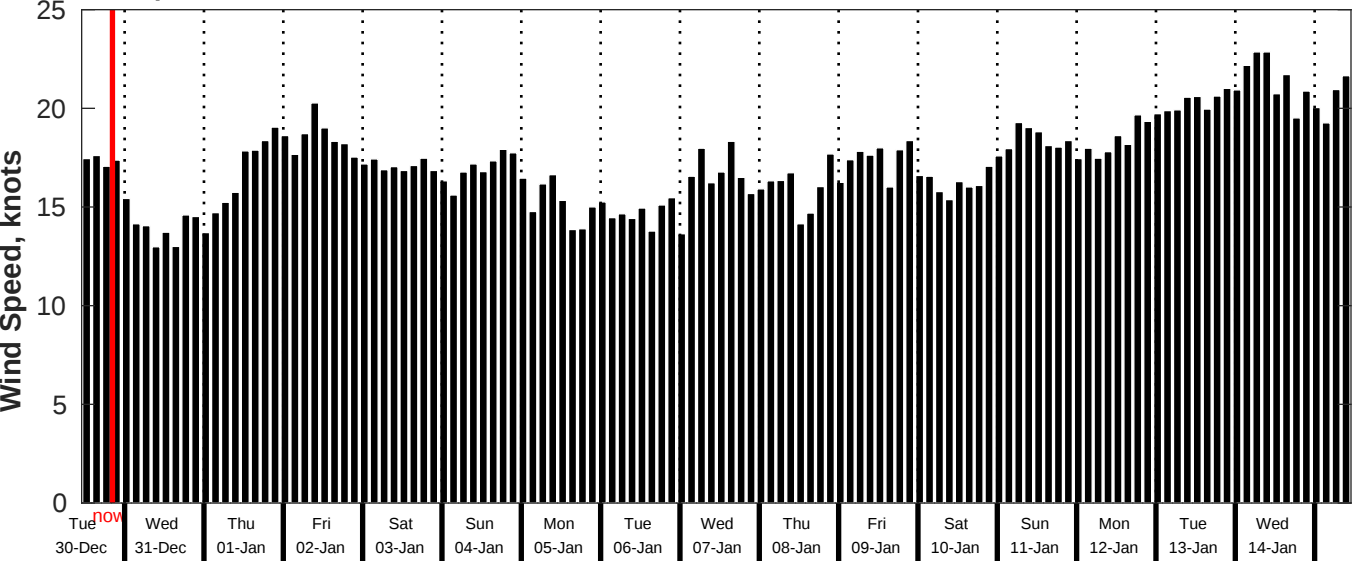
GFS Wind Speed Forecast for NDBC 52213 from 29-Dec-2025 11:00:00 to 14-Jan-2026 11:00:00
