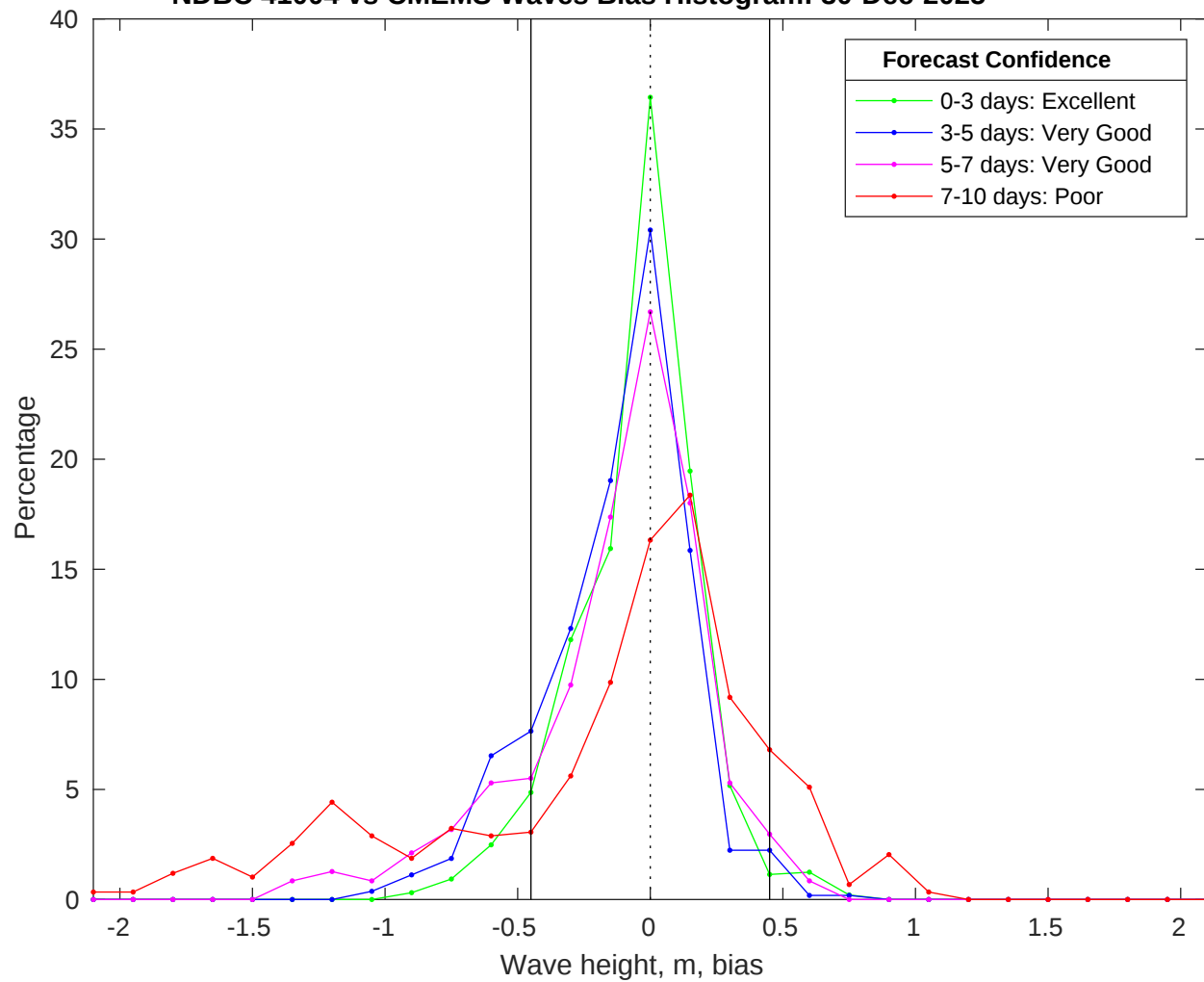
NDBC 41004 vs CMEMS Waves Bias Histogram: 30-Dec-2025
