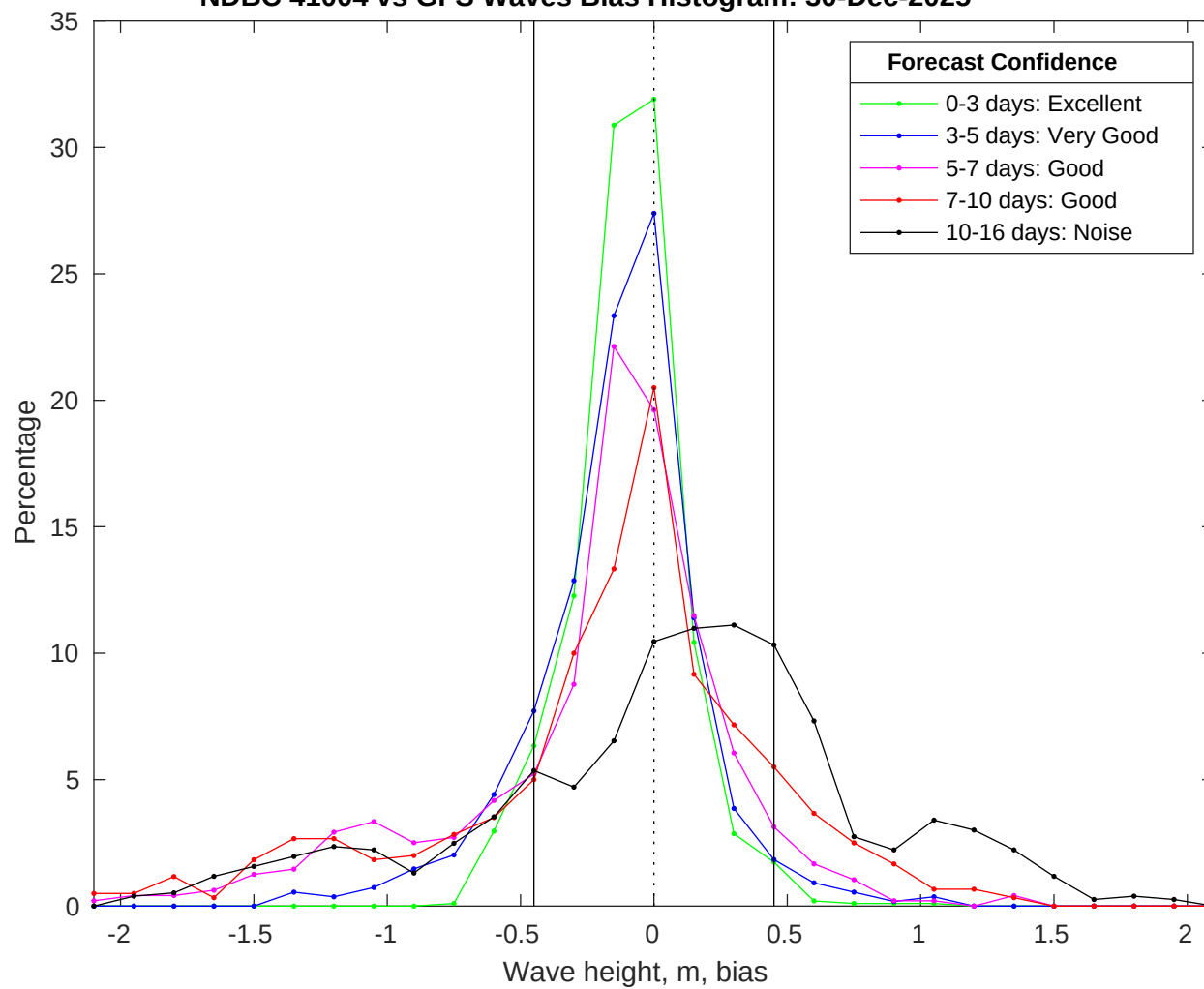
NDBC 41004 vs GFS Waves Bias Histogram: 30-Dec-2025
