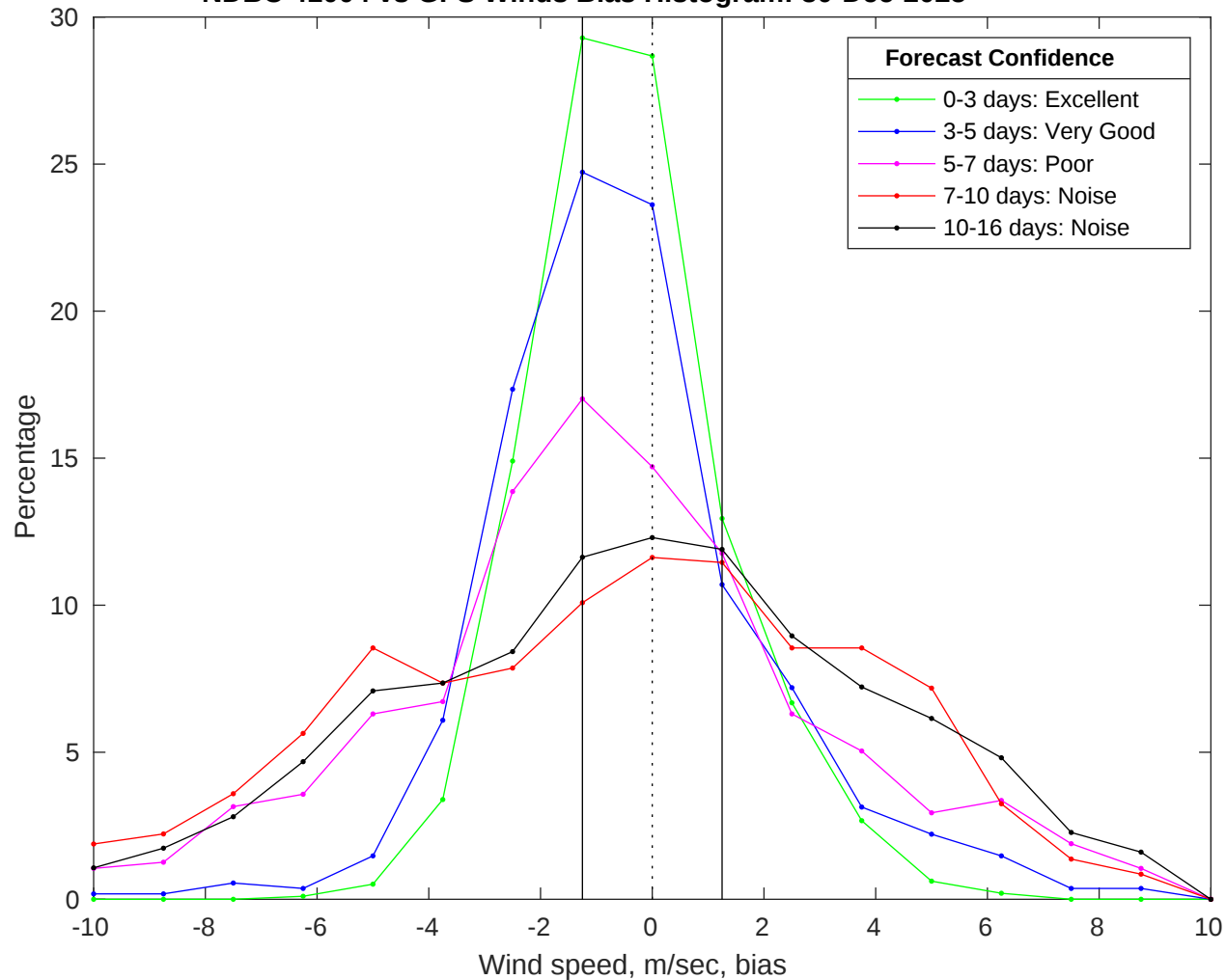
NDBC 41004 vs GFS Winds Bias Histogram: 30-Dec-2025
