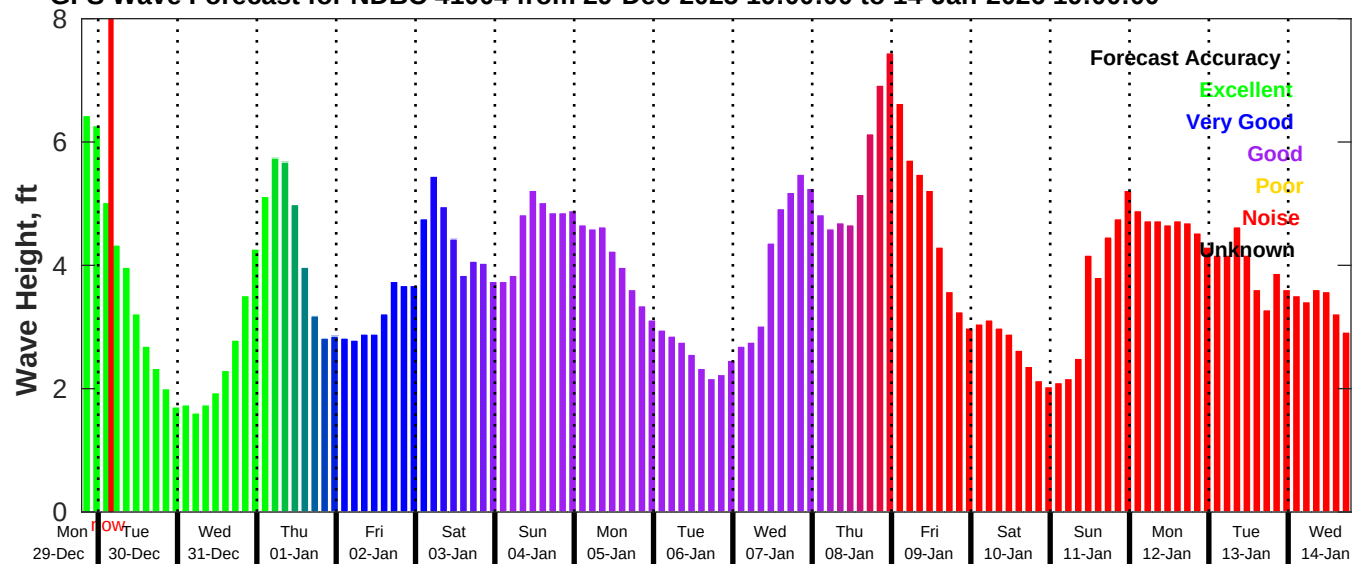
GFS Wave Forecast for NDBC 41004 from 29-Dec-2025 19:00:00 to 14-Jan-2026 19:00:00
