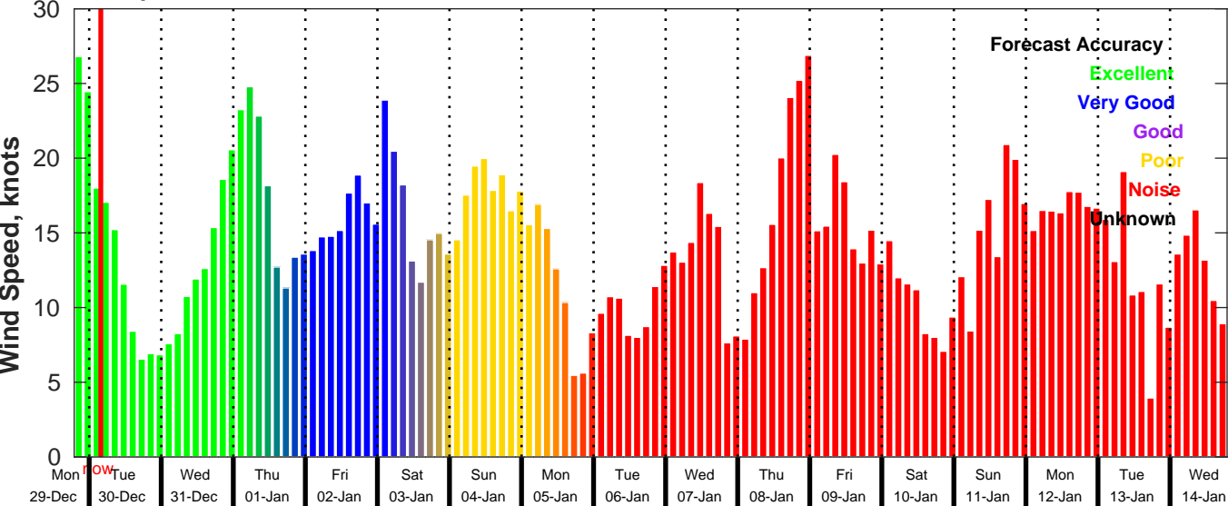
GFS Wind Speed Forecast for NDBC 41004 from 29-Dec-2025 19:00:00 to 14-Jan-2026 19:00:00
