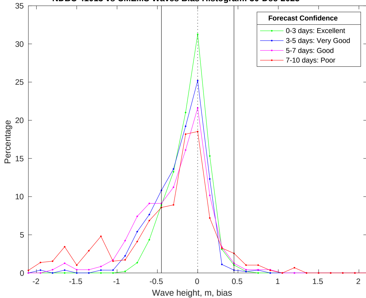
NDBC 41013 vs CMEMS Waves Bias Histogram: 30-Dec-2025
