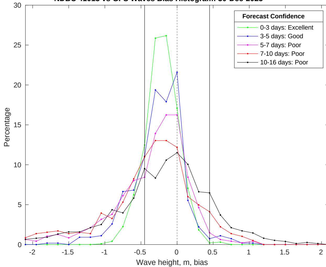
NDBC 41013 vs GFS Waves Bias Histogram: 30-Dec-2025
