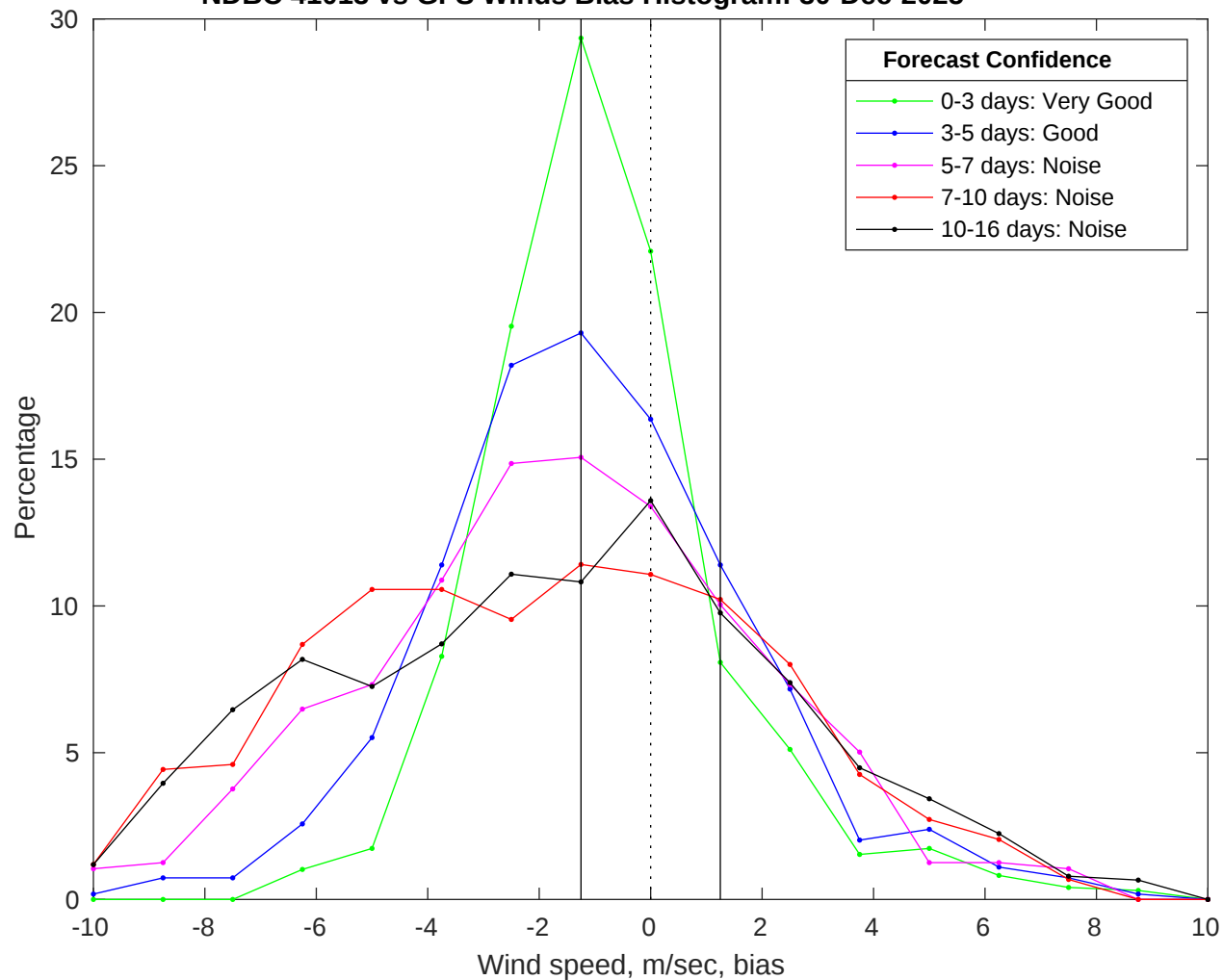
NDBC 41013 vs GFS Winds Bias Histogram: 30-Dec-2025
