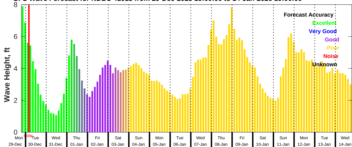
GFS Wave Forecast for NDBC 41013 from 29-Dec-2025 19:00:00 to 14-Jan-2026 19:00:00
