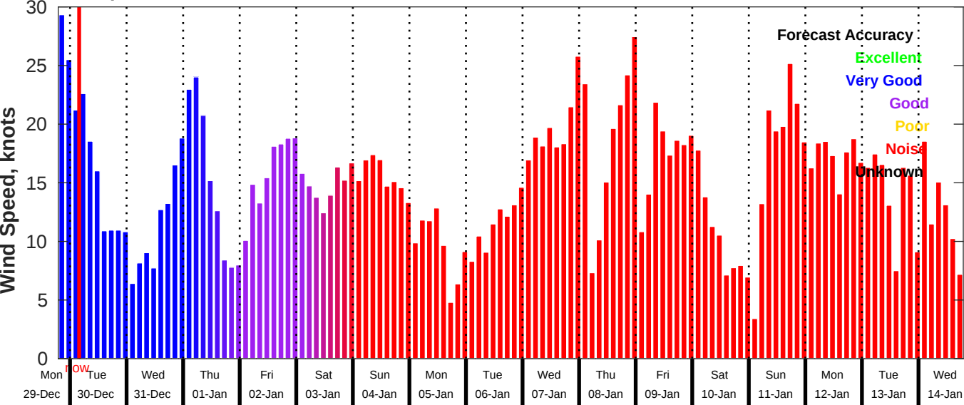
GFS Wind Speed Forecast for NDBC 41013 from 29-Dec-2025 19:00:00 to 14-Jan-2026 19:00:00
