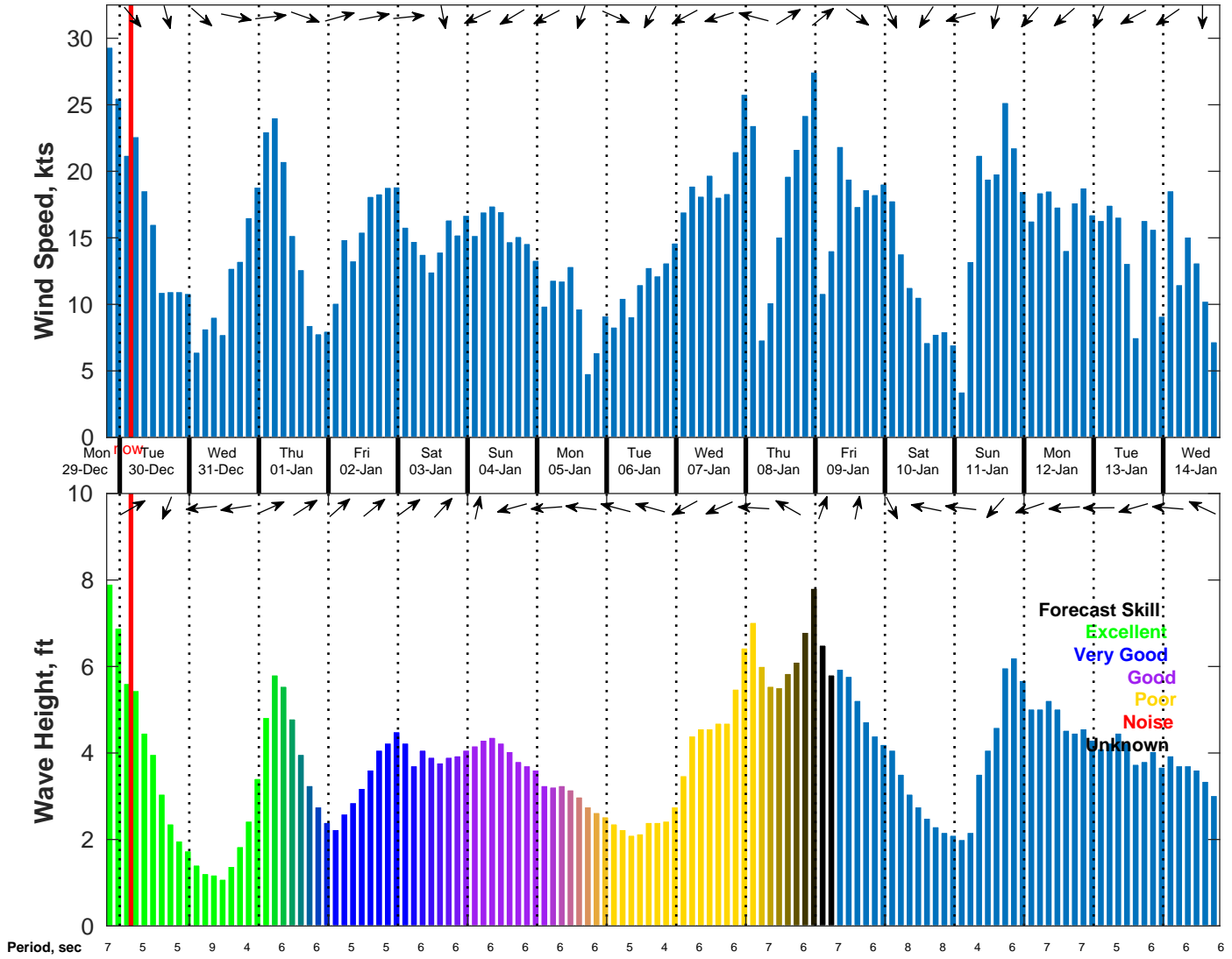
Wind & Wave Forecast for NDBC 41013 from 29-Dec-2025 19:00:00 to 14-Jan-2026 19:00:00
