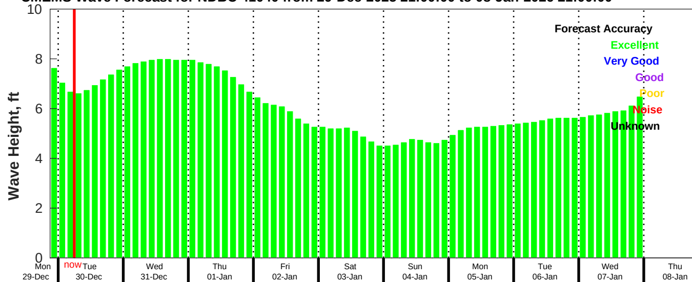
CMEMS Wave Forecast for NDBC 41040 from 29-Dec-2025 21:00:00 to 08-Jan-2026 21:00:00
