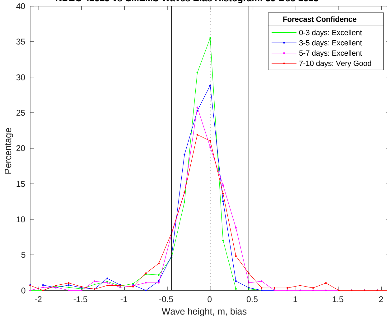
NDBC 42019 vs CMEMS Waves Bias Histogram: 30-Dec-2025
