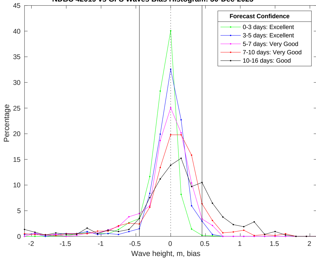
NDBC 42019 vs GFS Waves Bias Histogram: 30-Dec-2025
