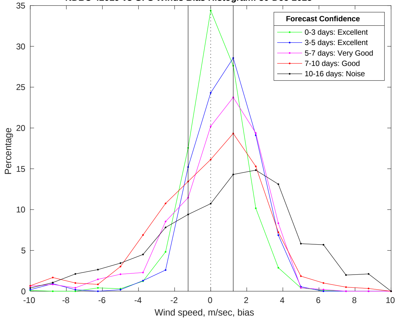
NDBC 42019 vs GFS Winds Bias Histogram: 30-Dec-2025
