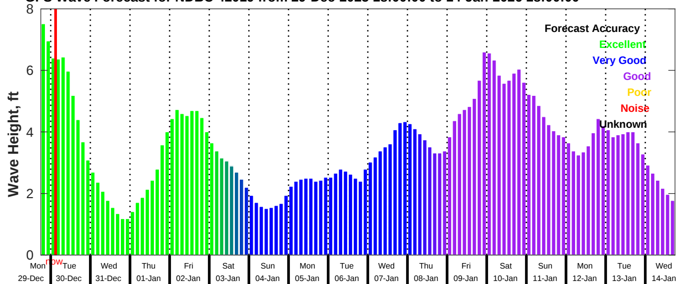
GFS Wave Forecast for NDBC 42019 from 29-Dec-2025 18:00:00 to 14-Jan-2026 18:00:00
