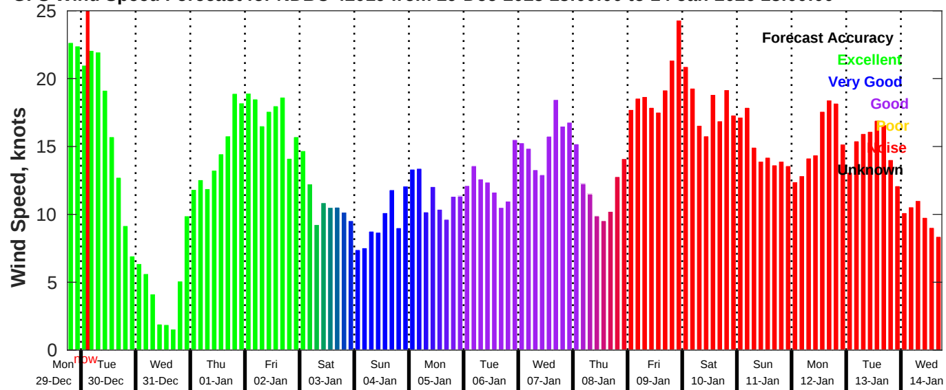
GFS Wind Speed Forecast for NDBC 42019 from 29-Dec-2025 18:00:00 to 14-Jan-2026 18:00:00
