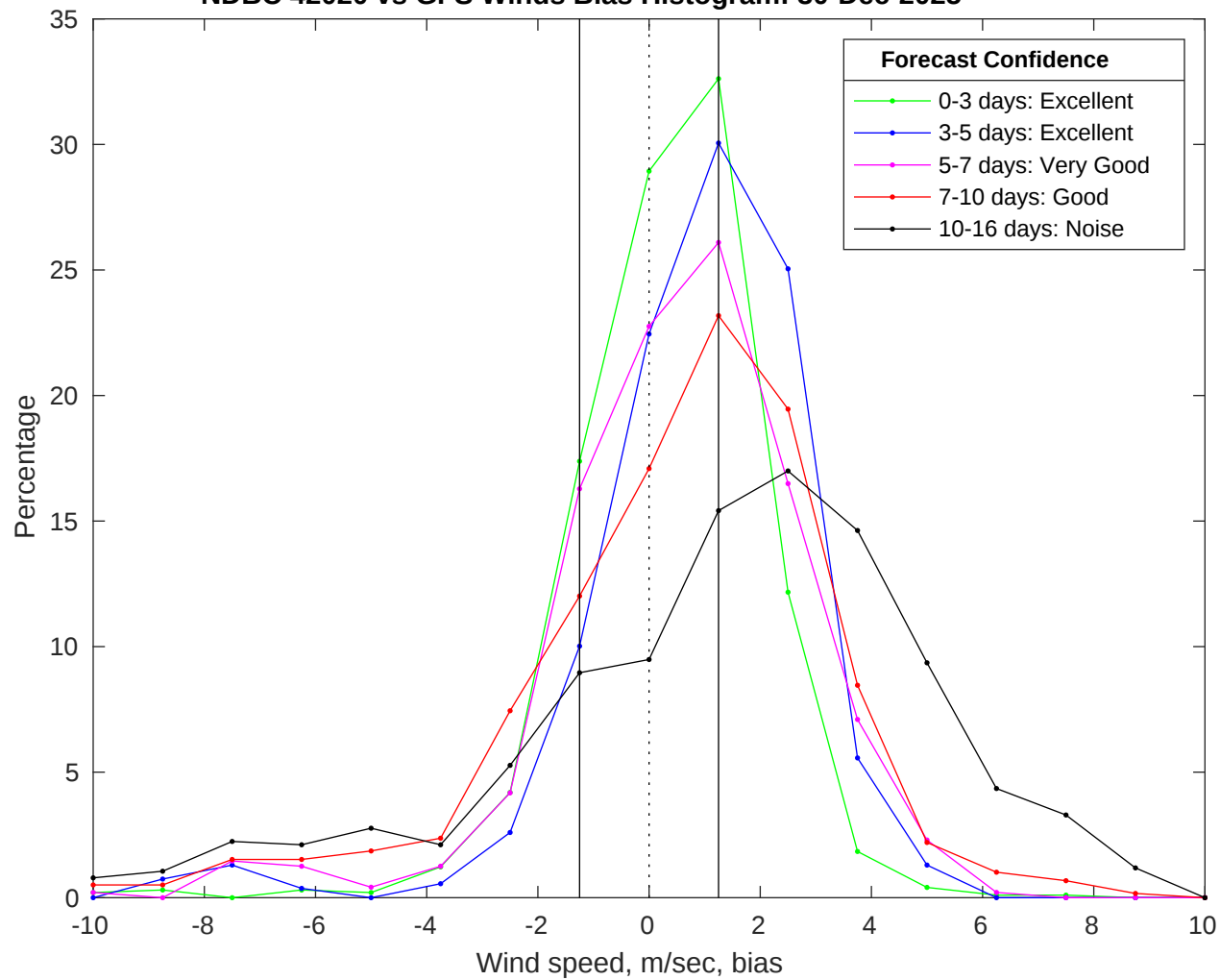
NDBC 42020 vs GFS Winds Bias Histogram: 30-Dec-2025
