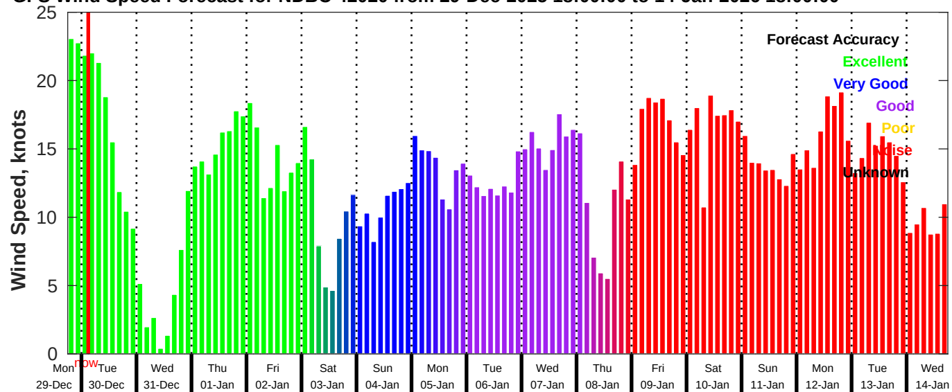
GFS Wind Speed Forecast for NDBC 42020 from 29-Dec-2025 18:00:00 to 14-Jan-2026 18:00:00
