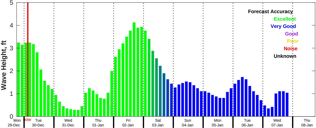
CMEMS Wave Forecast for NDBC 42035 from 29-Dec-2025 18:00:00 to 08-Jan-2026 18:00:00
