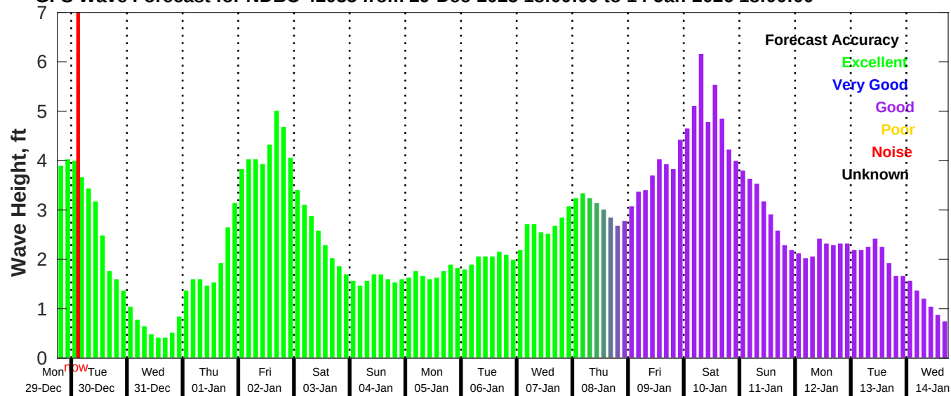
GFS Wave Forecast for NDBC 42035 from 29-Dec-2025 18:00:00 to 14-Jan-2026 18:00:00
