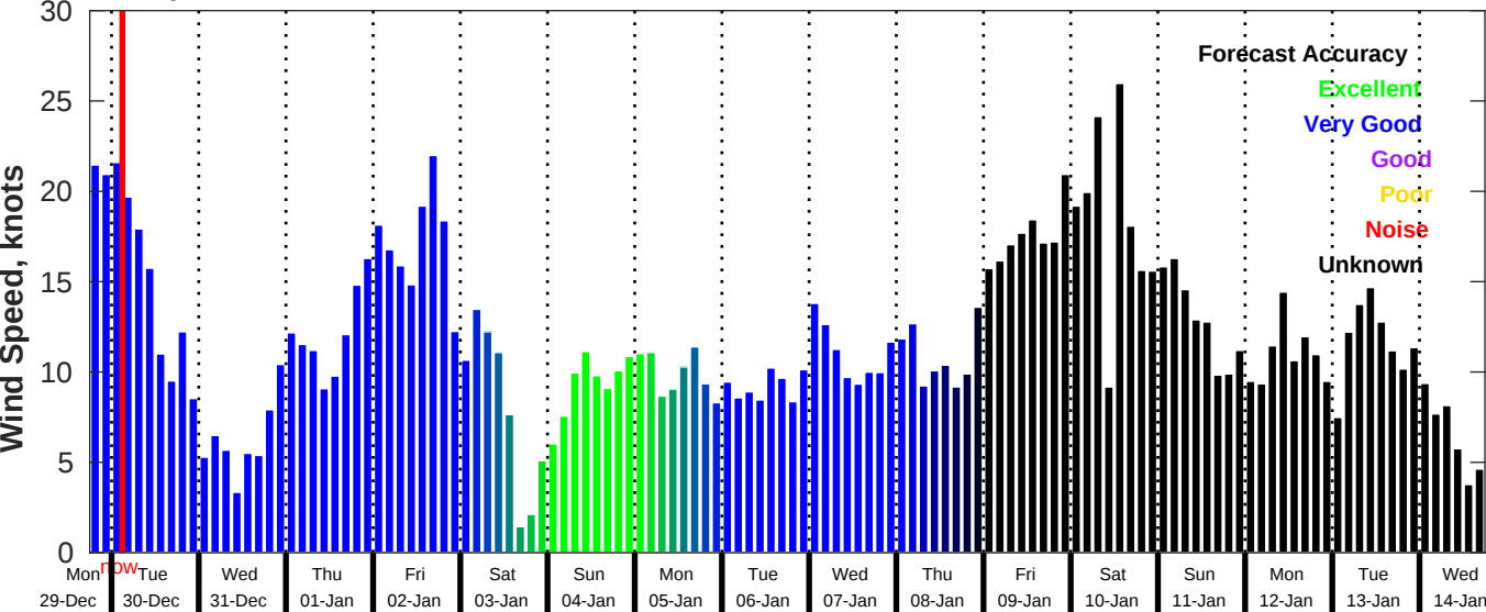
GFS Wind Speed Forecast for NDBC 42035 from 29-Dec-2025 18:00:00 to 14-Jan-2026 18:00:00
