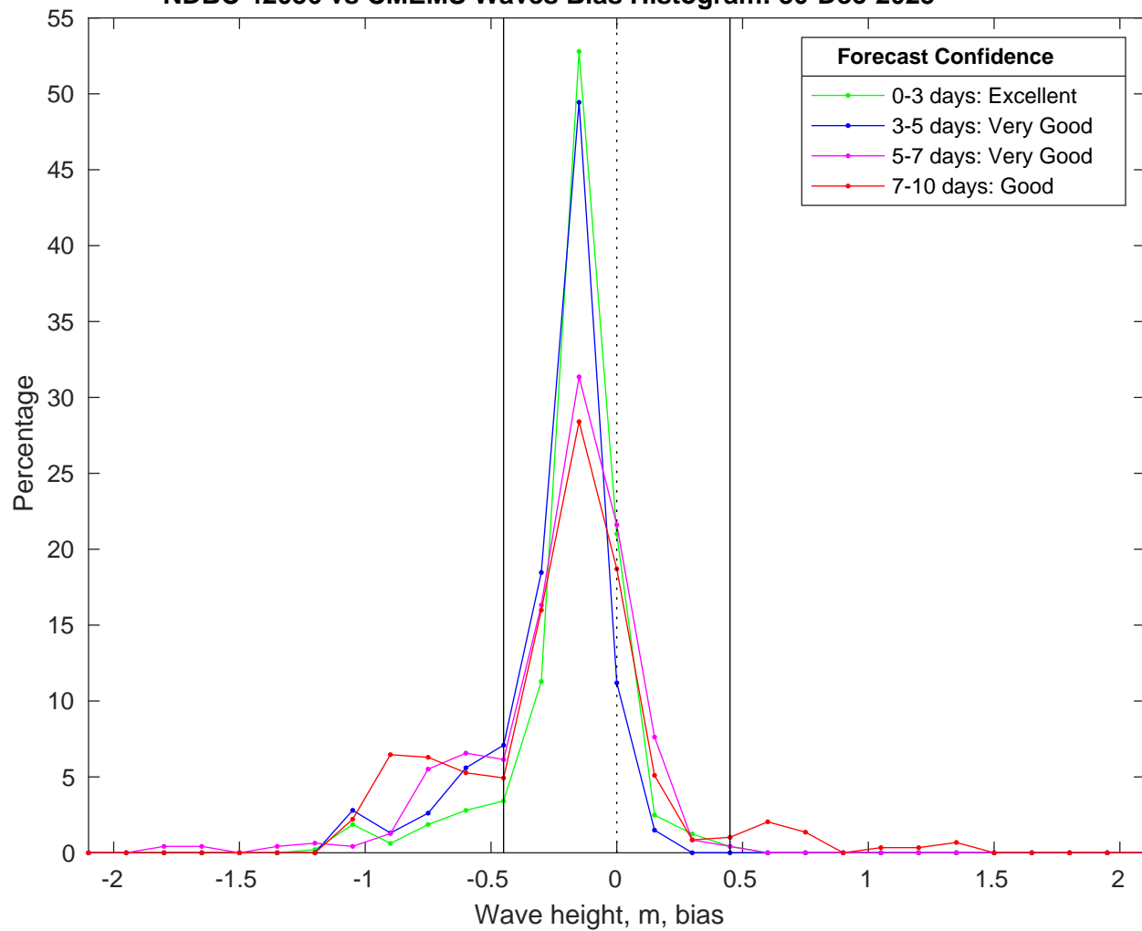
NDBC 42036 vs CMEMS Waves Bias Histogram: 30-Dec-2025
