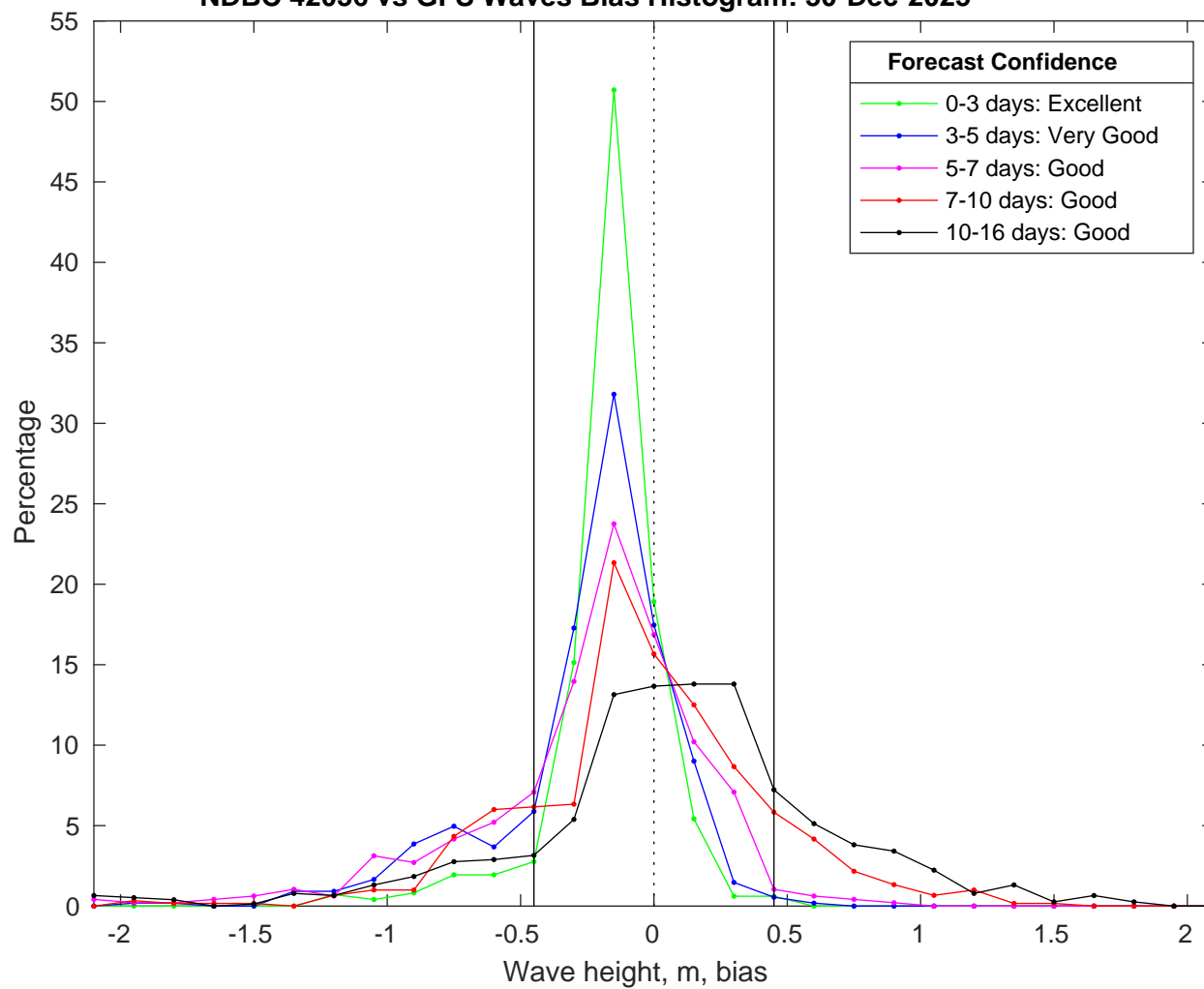
NDBC 42036 vs GFS Waves Bias Histogram: 30-Dec-2025
