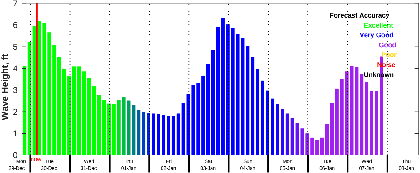
CMEMS Wave Forecast for NDBC 42036 from 29-Dec-2025 19:00:00 to 08-Jan-2026 19:00:00
