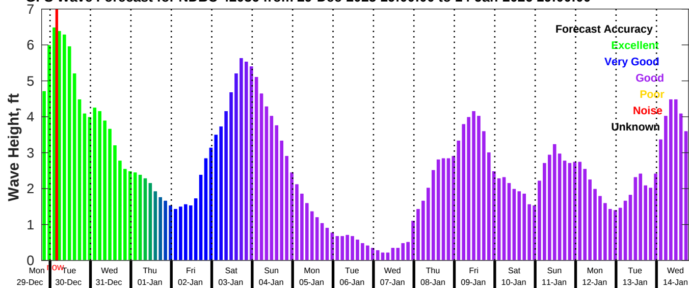
GFS Wave Forecast for NDBC 42036 from 29-Dec-2025 19:00:00 to 14-Jan-2026 19:00:00
