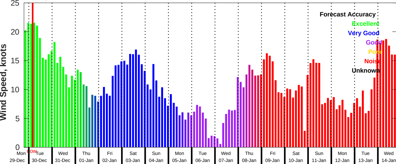
GFS Wind Speed Forecast for NDBC 42036 from 29-Dec-2025 19:00:00 to 14-Jan-2026 19:00:00
