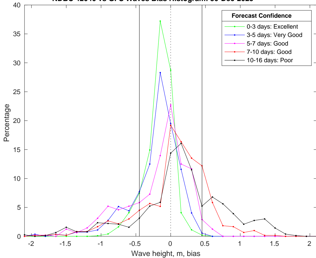
NDBC 42040 vs GFS Waves Bias Histogram: 30-Dec-2025
