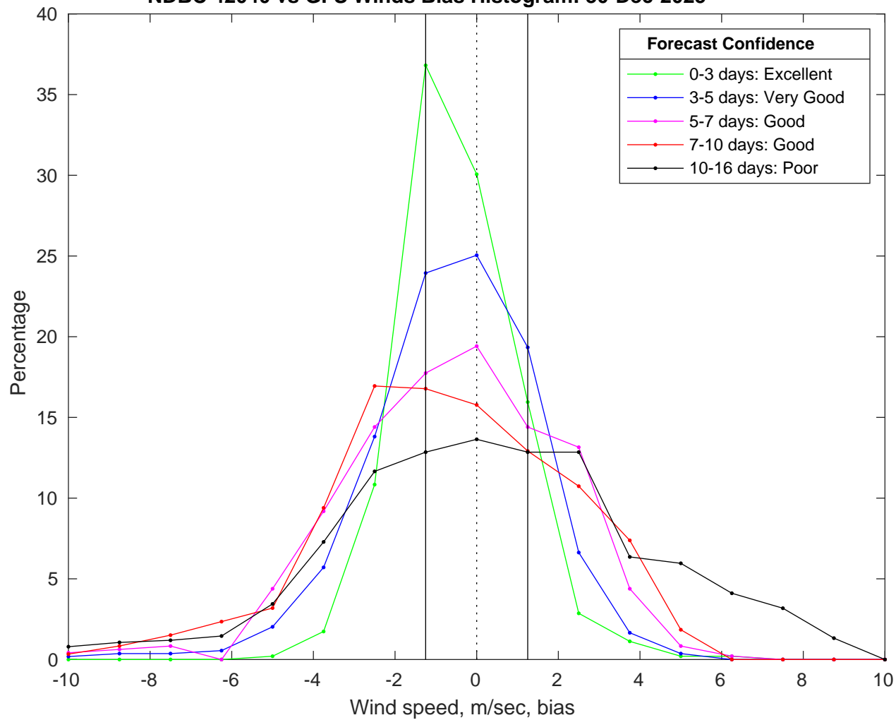
NDBC 42040 vs GFS Winds Bias Histogram: 30-Dec-2025
