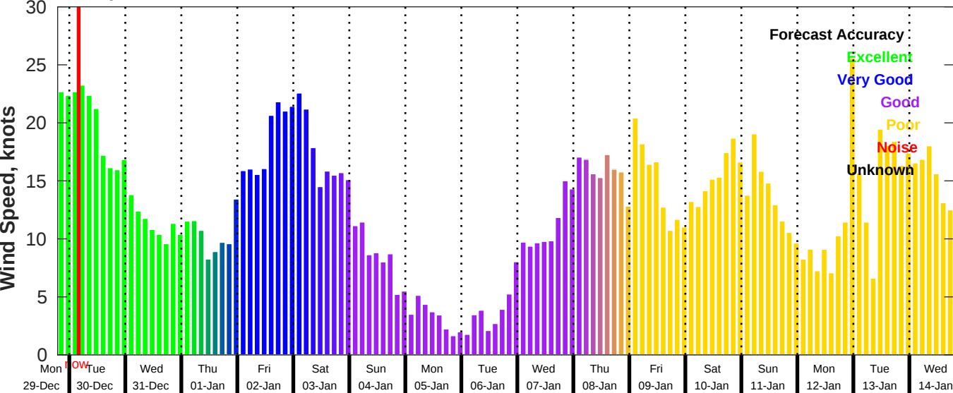
GFS Wind Speed Forecast for NDBC 42040 from 29-Dec-2025 19:00:00 to 14-Jan-2026 19:00:00
