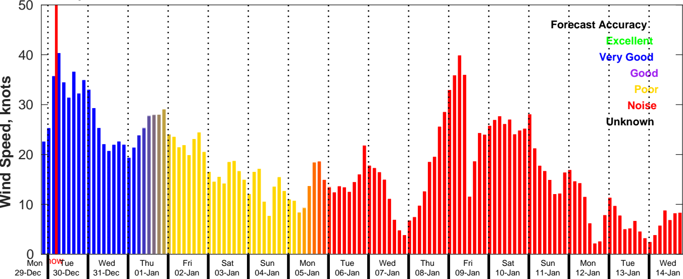
GFS Wind Speed Forecast for NDBC 44008 from 29-Dec-2025 20:00:00 to 14-Jan-2026 20:00:00
