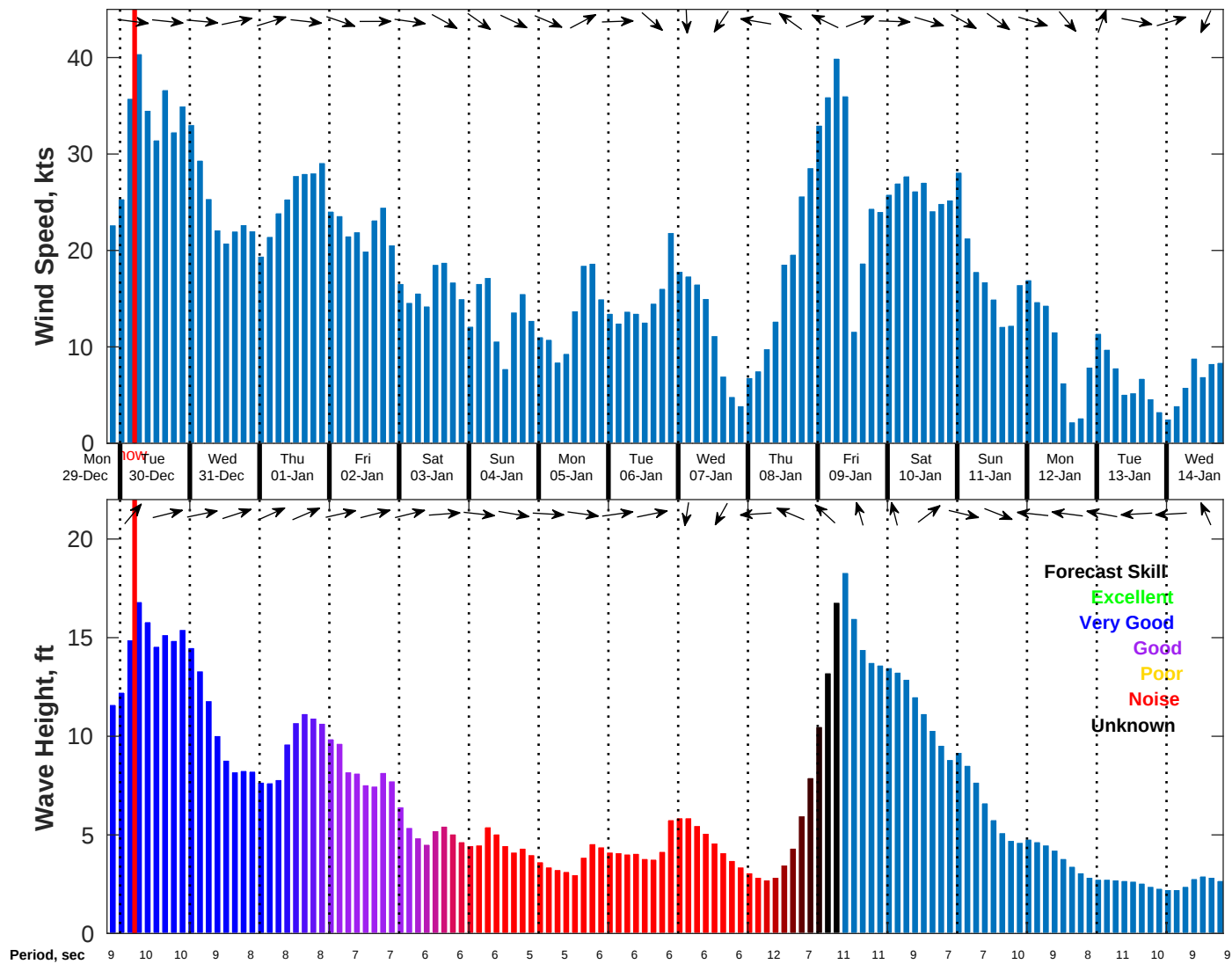
Wind & Wave Forecast for NDBC 44008 from 29-Dec-2025 20:00:00 to 14-Jan-2026 20:00:00
