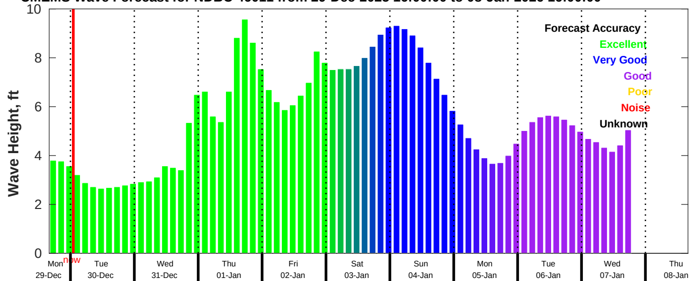
CMEMS Wave Forecast for NDBC 46011 from 29-Dec-2025 16:00:00 to 08-Jan-2026 16:00:00
