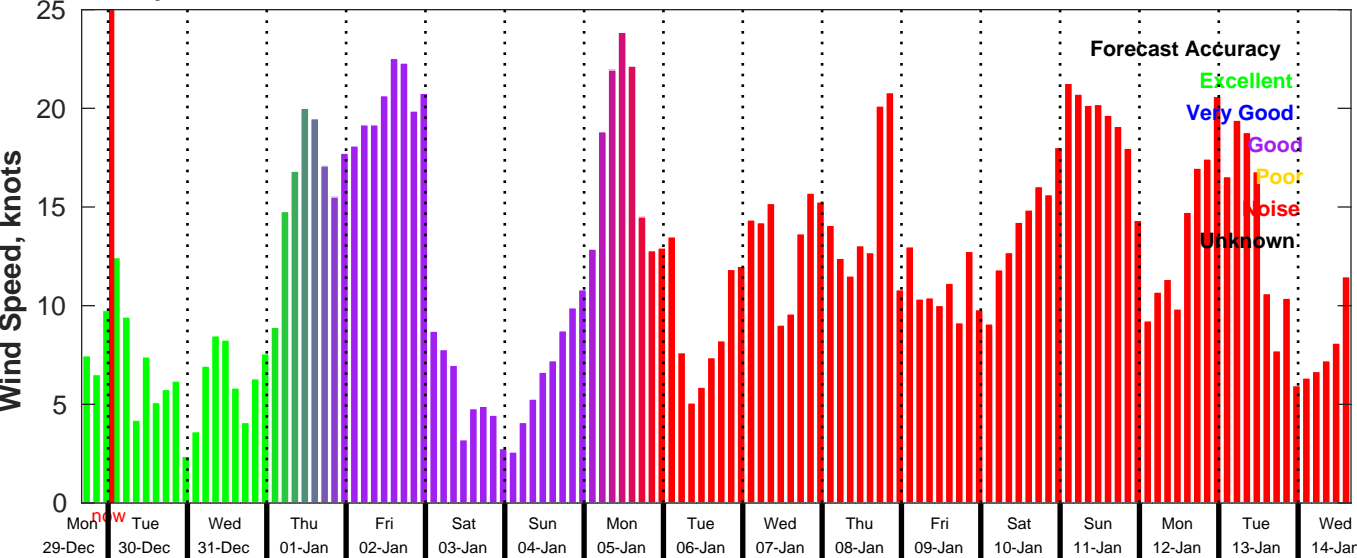
GFS Wind Speed Forecast for NDBC 46011 from 29-Dec-2025 16:00:00 to 14-Jan-2026 16:00:00
