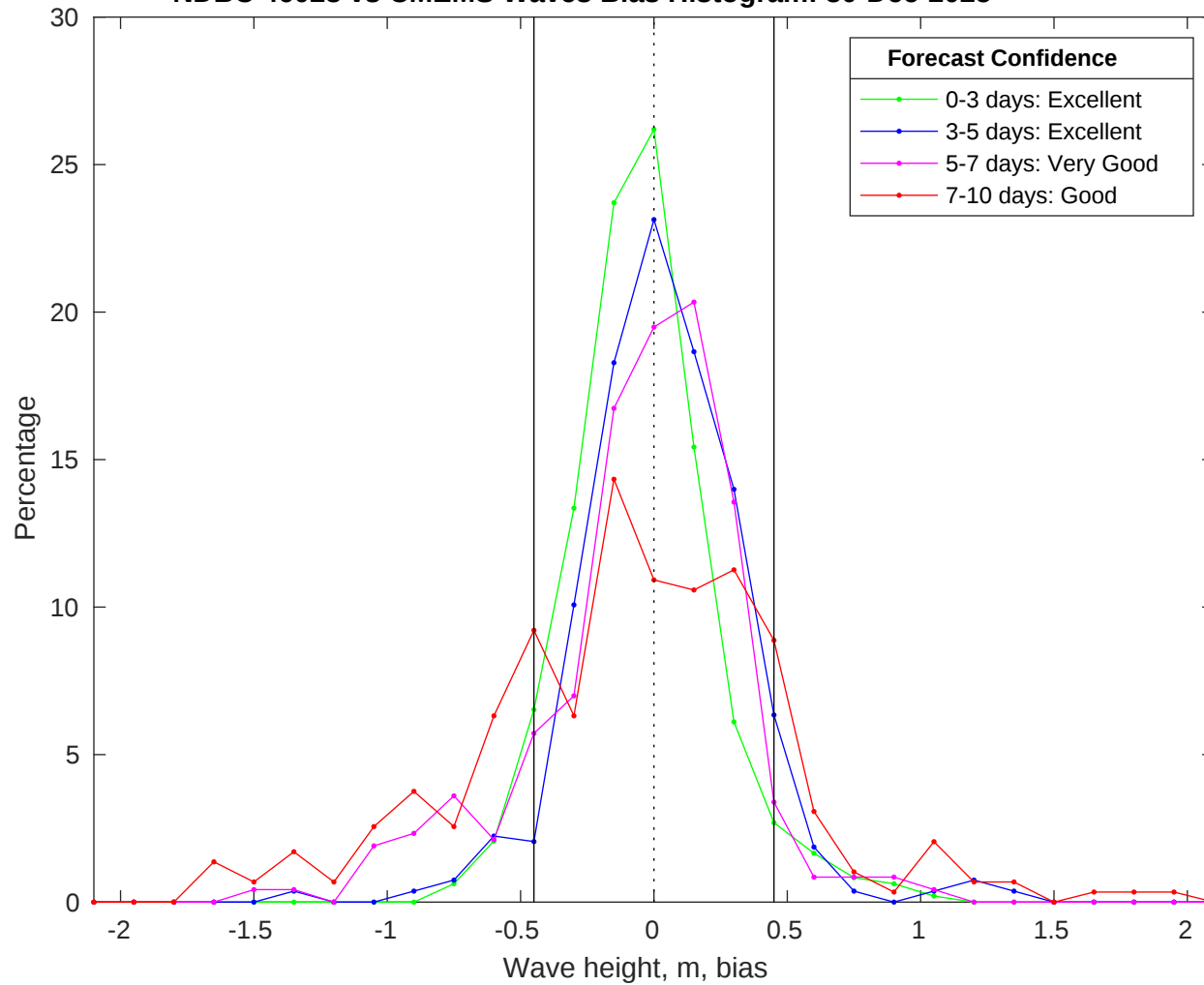
NDBC 46028 vs CMEMS Waves Bias Histogram: 30-Dec-2025
