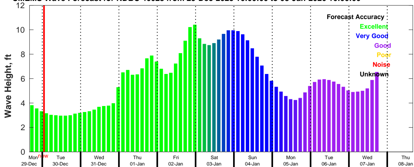
CMEMS Wave Forecast for NDBC 46028 from 29-Dec-2025 16:00:00 to 08-Jan-2026 16:00:00
