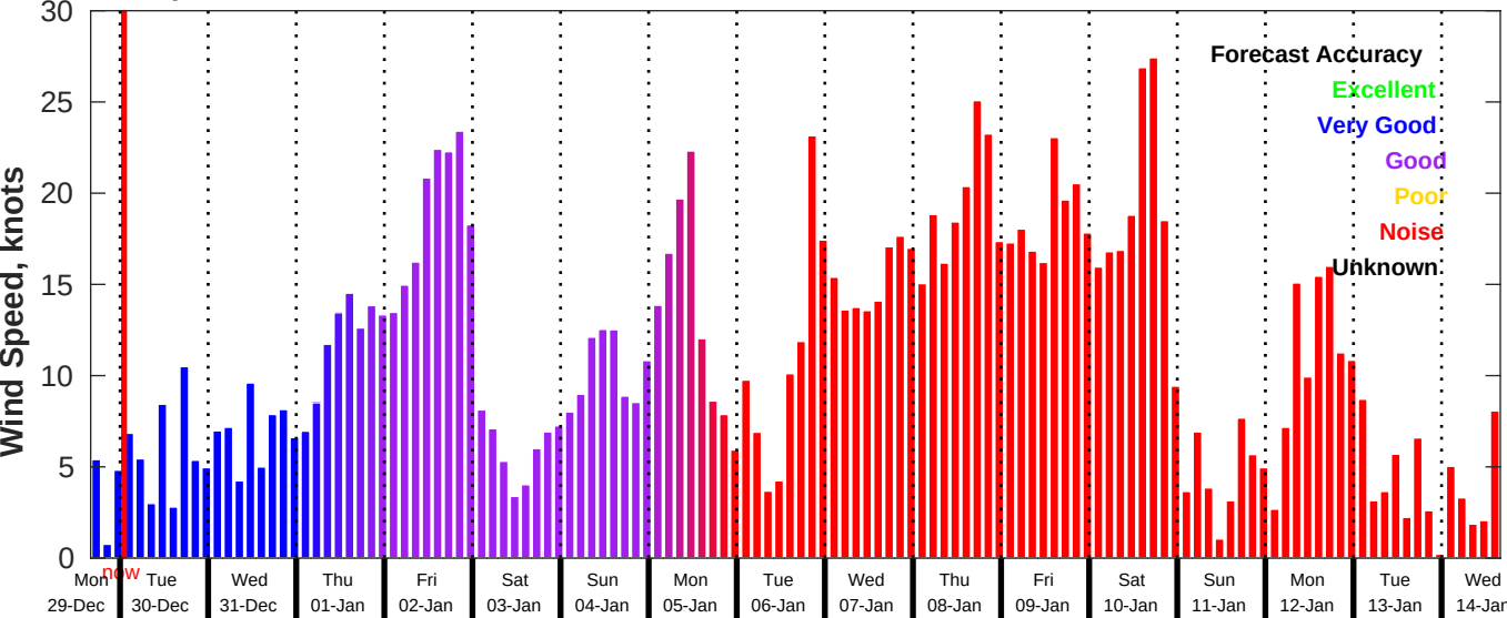
GFS Wind Speed Forecast for NDBC 46028 from 29-Dec-2025 16:00:00 to 14-Jan-2026 16:00:00
