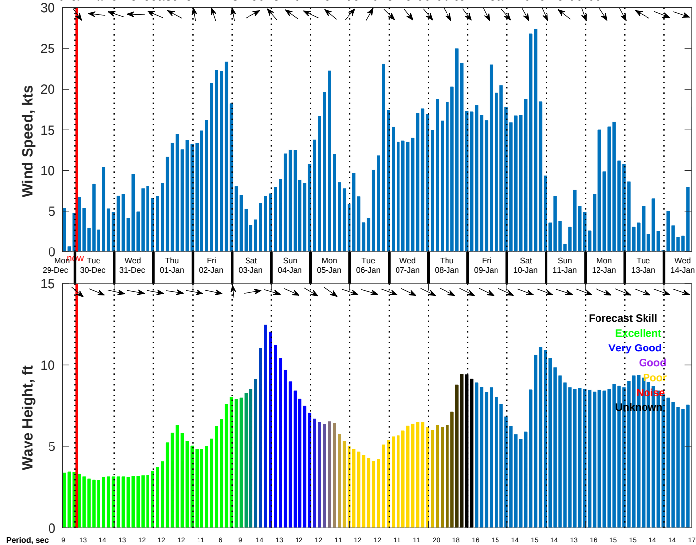
Wind & Wave Forecast for NDBC 46028 from 29-Dec-2025 16:00:00 to 14-Jan-2026 16:00:00
