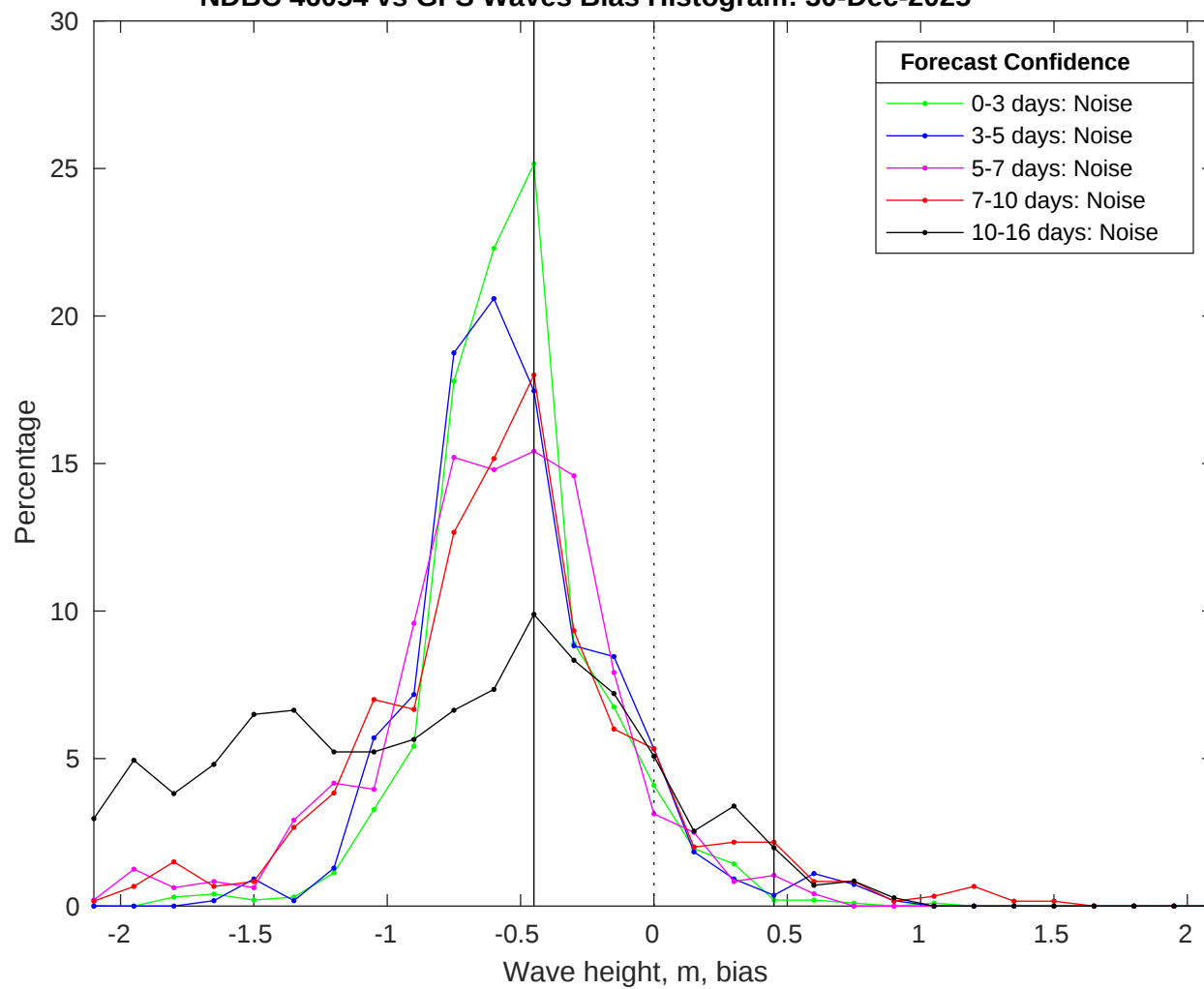
NDBC 46054 vs GFS Waves Bias Histogram: 30-Dec-2025
