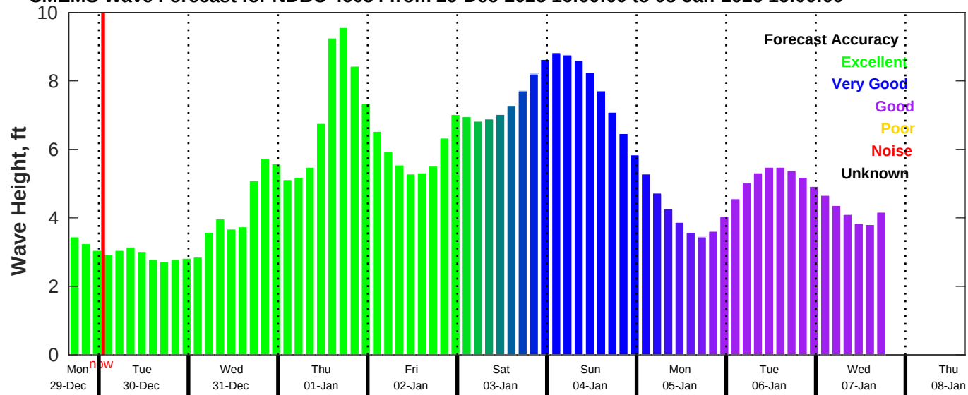
CMEMS Wave Forecast for NDBC 46054 from 29-Dec-2025 16:00:00 to 08-Jan-2026 16:00:00
