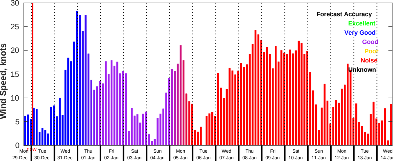
GFS Wind Speed Forecast for NDBC 46054 from 29-Dec-2025 16:00:00 to 14-Jan-2026 16:00:00
