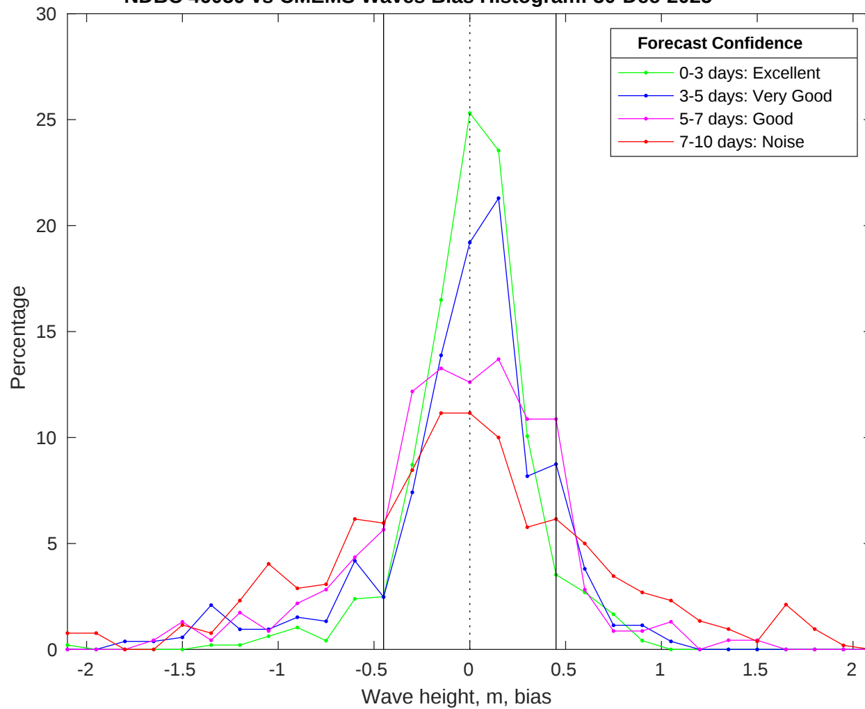
NDBC 46059 vs CMEMS Waves Bias Histogram: 30-Dec-2025
