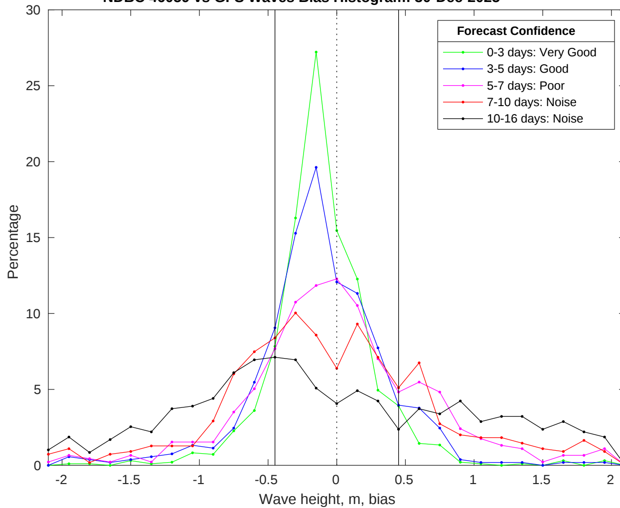
NDBC 46059 vs GFS Waves Bias Histogram: 30-Dec-2025
