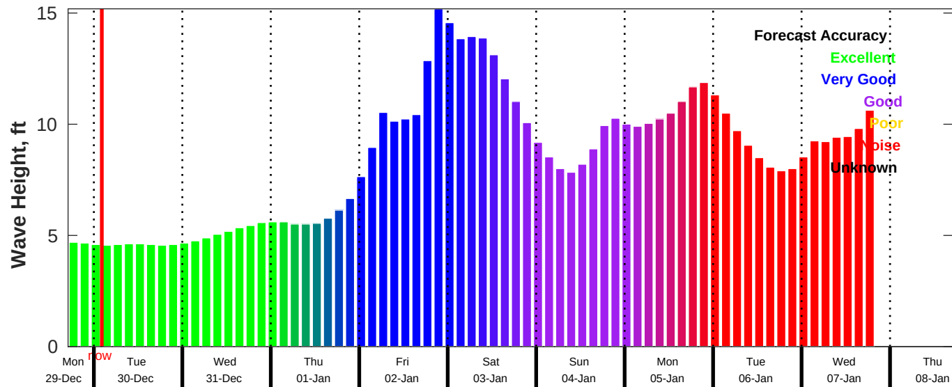
CMEMS Wave Forecast for NDBC 46059 from 29-Dec-2025 17:00:00 to 08-Jan-2026 17:00:00
